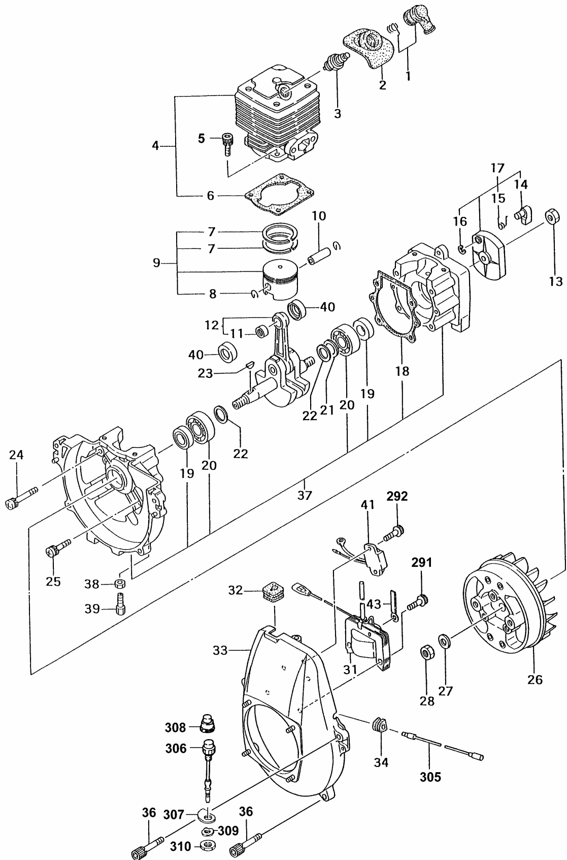
FIG—1 CYLINDER PISTON CRANCASE
